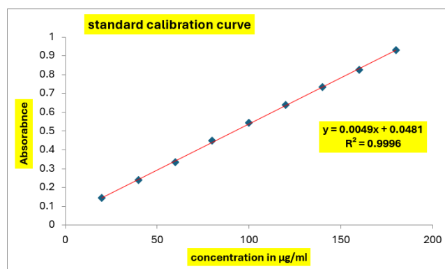
Figure 6: Calibration Curve of The Proposed Method
