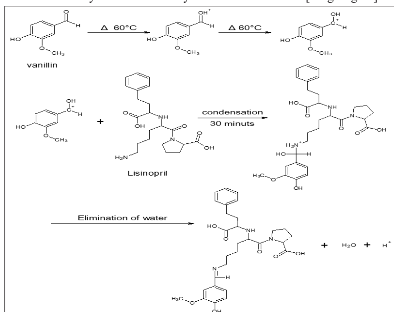
Figure 7: Proposed Lisinopril-Vanillin Reaction Mechanism
