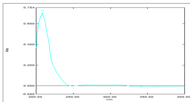
Figure 4: UV Spectrum of Lisinopril Solution in Methanol
