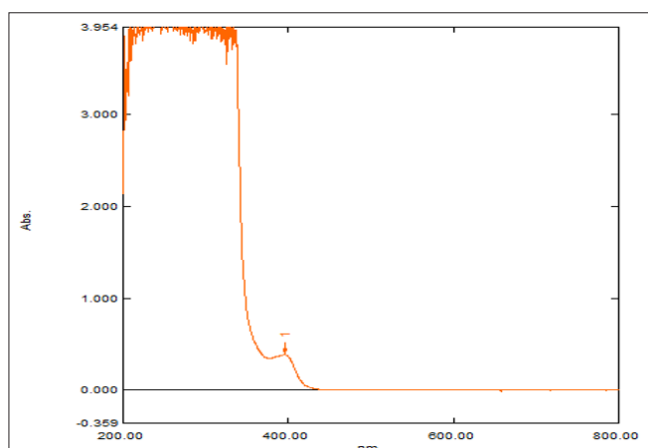
Figure 3: Spectrum of Lisinopril and Vanillin Mixture
