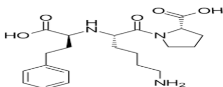
Figure 1: Chemical Structure of Lisinopril
