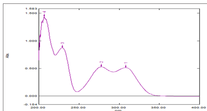
Figure 5: UV Spectrum of Vanillin in Methanol Linearity
