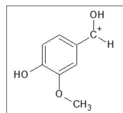
Figure 2: Chemical Structure of Vanillin
