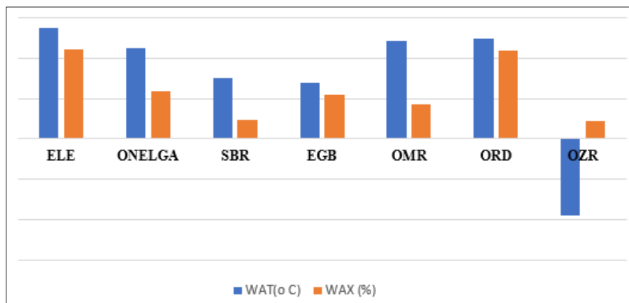
Figure 13: Wax Against WAT Profile for Waxy Crude Samples
