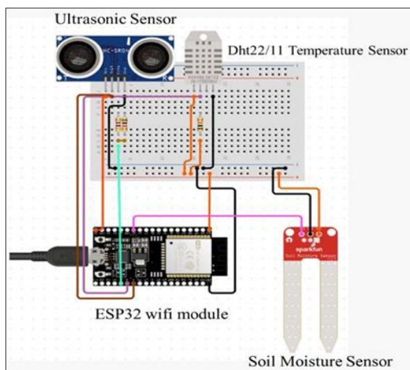
Figure 10: Circuit Diagram for Unfiltered Tank
