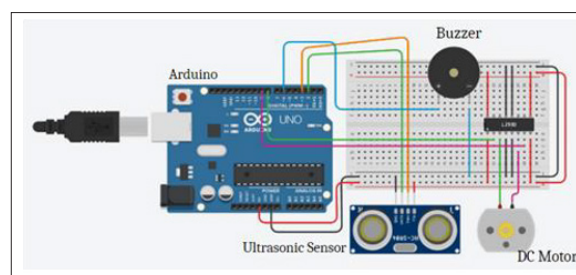
Figure 12: Circuit Diagram for Home Water Tank
