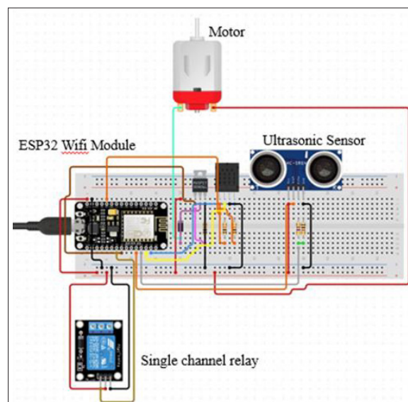
Figure 11: Circuit Diagram for Filtered Tank
