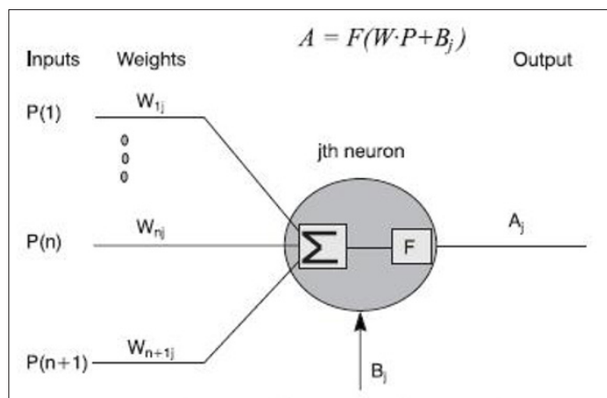
Figure 1: Neural network equation Source: Otero (1988)
