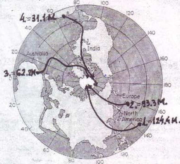
FIG. 30. Unsuccessful attempts to explain palaeomagnetic data by means of the pole-wandering hypothesis (after Heezen).
