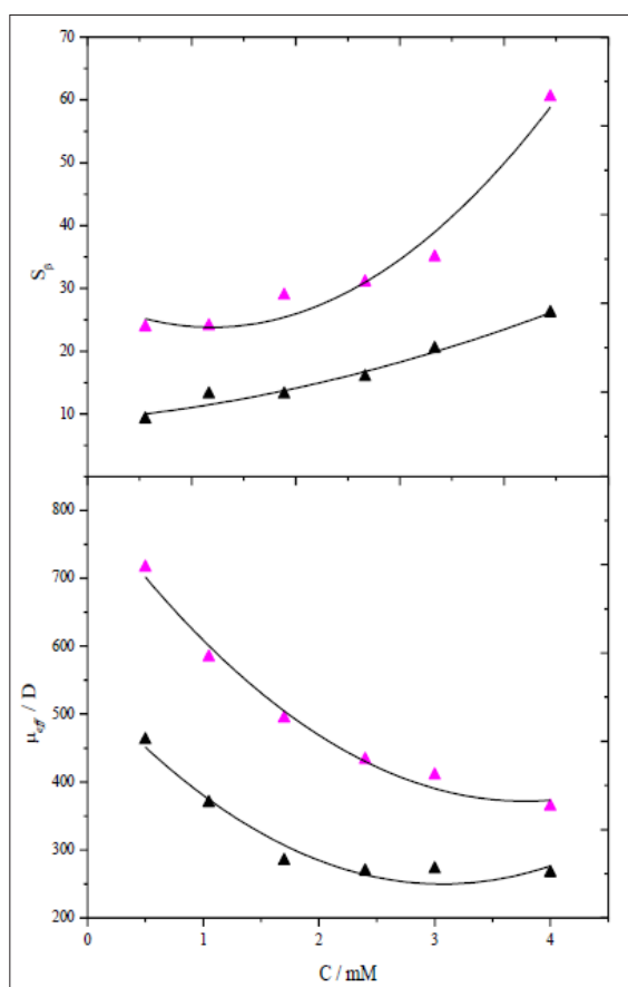
Figure 4: Amplitude, S_0 , and effective dipole moment, \mu_{\text{eff}} , for LYS interacting with holo \alpha -LA (black) and apo \alpha -LA (magenta) at various complex concentration. Lines are for visualization only.
