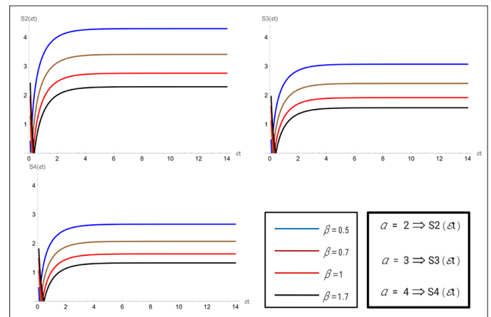
Figure 4: Plot of expressions (4.12)
