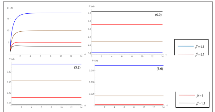
Figure 3: Plot of expressions (4.7) and (4.8). The couple (m_0, n_0) for example m_0 = 3 , n_0 = 2 are denoted (3, 2).
