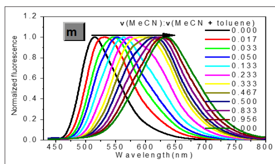
Figure S8: Normalized one-photon emission spectra of 1a ( c = 10^{-5} M, \lambda_{ex} = 410 nm) in toluene-MeCN mixture versus MeCN concentrations
