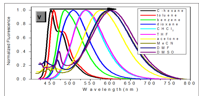
Figure S14: Normalized one-photon emission spectra of 1b ( c = 10^{-6} M, \lambda_{\text{ex}} = 412 nm) in various solvents
