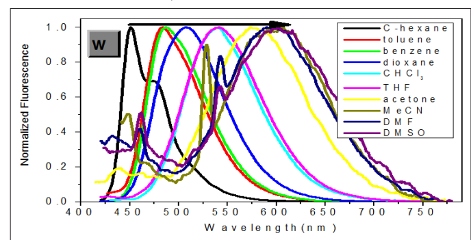
Figure S15: Normalized two-photon emission spectra of 1b ( c = 10^{-6} M, \lambda_{\text{ex}} = 810 nm) in various solvents
