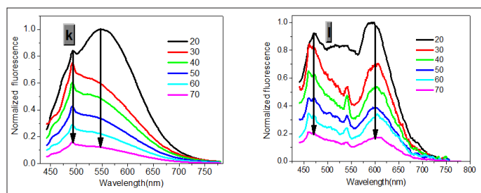
Figure S7: Normalized (k) one- ( \lambda_{ex} = 410 nm) and (l) two-photon ( \lambda_{ex} = 790 nm) emission spectra of 1a ( c = 10^{-6} M) in glycerol versus temperature ( ^{\circ}\text{C} ).
