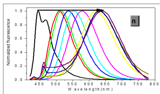
Figure S9: Normalized two-photon emission spectra (left to right: C-hexane, toluene, benzene, dioxane, \text{CHCl}_3 , THF, acetone, MeCN, DMF, DMSO) of 1a ( c = 10^{-5} M, \lambda_{ex} = 790 nm) in various solvents.
