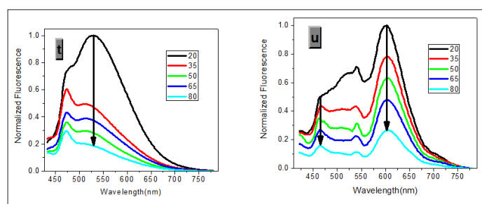
Figure S13: Normalized (t) one- ( \lambda_{\text{ex}} = 410 nm) and (u) two-photon ( \lambda_{\text{ex}} = 790 nm) emission spectra of 1b ( c = 10^{-6} M) in glycerol versus temperature ( ^{\circ}\text{C} ).
