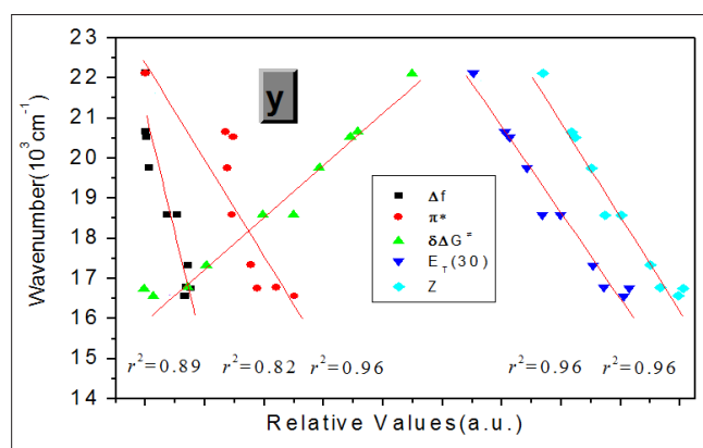
Figure S17: Correlation between the emission maxima (in \text{cm}^{-1} ) of 1b ( c = 10^{-6} M, \lambda_{\text{ex}} = 412 nm) in various solvents and selected solvent parameters such as \Delta f , \pi^* , \delta\Delta G^\ddagger , E_T(30) and Z .
