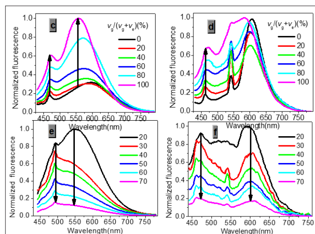
Figure 2: Normalized (c) one- and (d) two-photon emission spectra of 1a ( c = 3 \times 10^{-6} M, \lambda_{\text{ex}}(\text{OP}) = 410 nm, \lambda_{\text{ex}}(\text{TP}) = 790 nm) in glycerol-ethanol ( v_g/(v_g+v_e) , %). Normalized (e) one- and (f) two-photon emission spectra of 1a ( c = 10^{-6} M, \lambda_{\text{ex}}(\text{OP}) = 410 nm, \lambda_{\text{ex}}(\text{TP}) = 790 nm) in glycerol versus temperature ( ^\circ\text{C} ).
