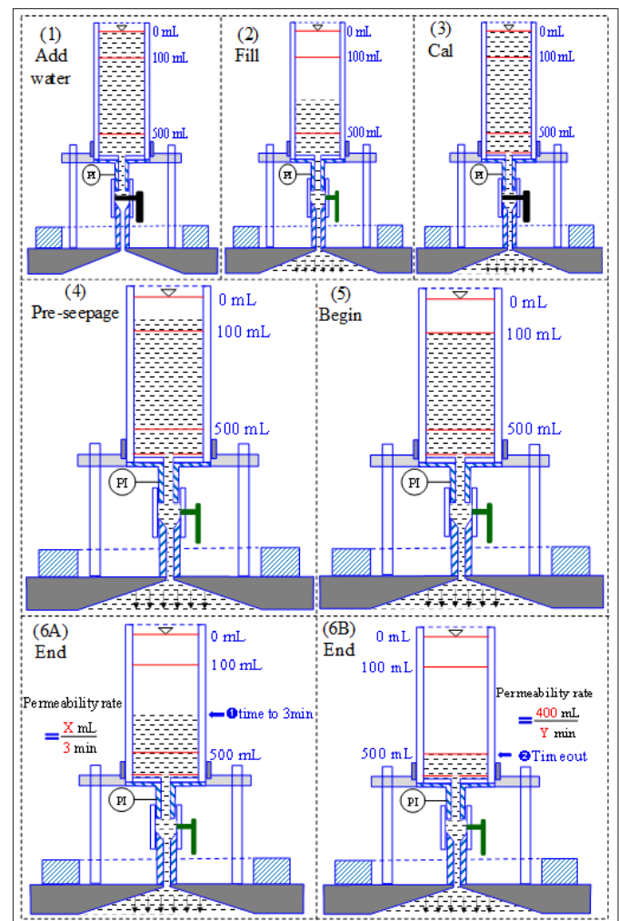
Figure 1: Schematic Diagram of the Process Steps
