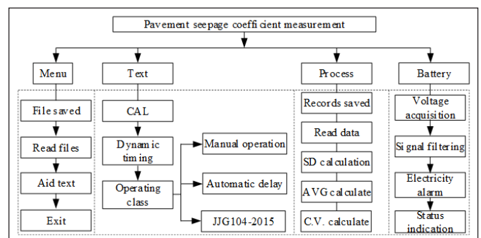
Figure 4: Functional Diagram of the Application Software
