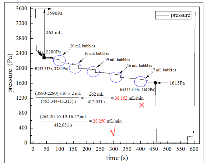
Figure 13: Curve of Bubble Burst Process
