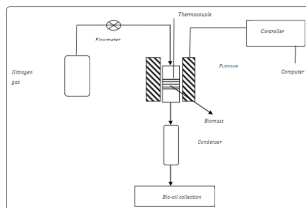
Figure 2.1: The tubular fixed bed reactor set-up
