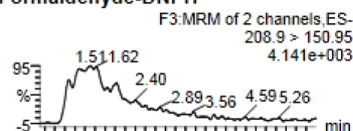
Fig 3: Chromatogram for Aglaonema, showing HCHO concentration on LCMS
