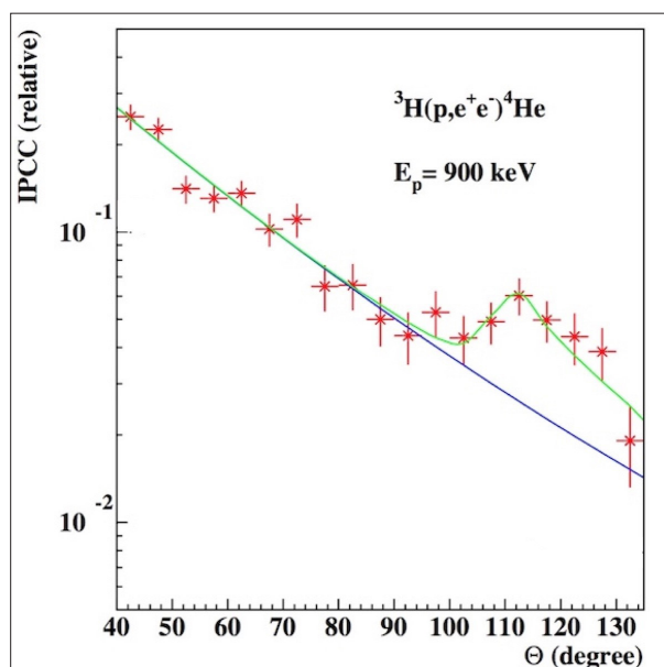
Figure 1: Angular correlations for the e^-e^+ pairs measured in the {}^3\text{H}(p,e^+e^-){}^4\text{He} reaction at E_p=900 keV. The red points are the experimental data showing the e^-e^+ pairs excess around 115^\circ . The blue is the expected angular distribution of e^-e^+ pairs based on standard IPC physics, while the green line is the best data fit assuming M_{X17}=16.87 MeV
