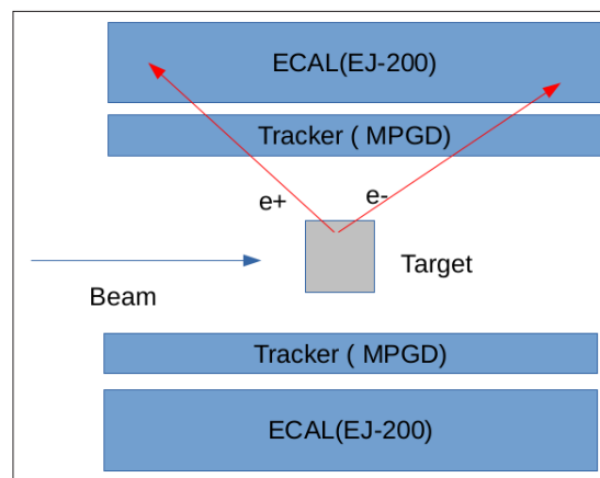
Figure 4: Conceptual design of the {}^3\text{He}(n,e^+e^-){}^4\text{He} at EAR2. The neutron beam strikes on a {}^3\text{He} target, done in special carbon fiber, 0.6 mm thick, 300 - 350 atm. The tracks direction are measured for the first 3 cm with the inner detector (TPC) then by the EJ-200 slab planes, the energy of each particle is measured with a e.m. calorimeter with adequate granularity (EJ-200).
