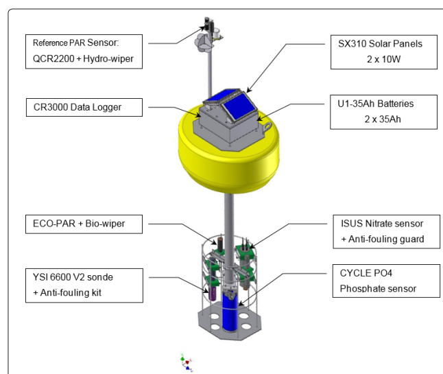
Figure 1: NDB with 10W Solar Panels
