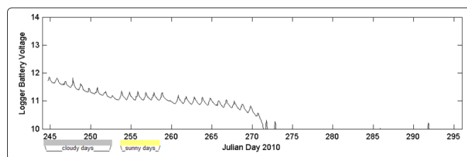
Figure 3: CR3000 Data Logger Battery Voltage
