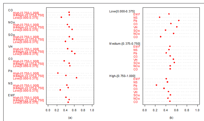
Figure 7: Probability of low control action demand for all pollutants, instantiated at low, medium and high level of risk perception and judgment. (a) Pollutants; (b) level
