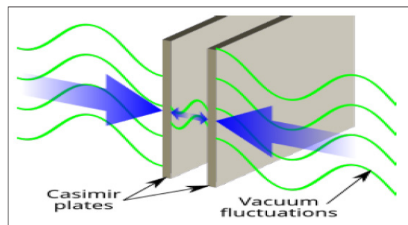
Figure 4: Casimir Effect
