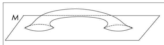
Figure 1: Schematic Image. Wormhole Manifold is attached from two components, the 'handle' and space with two holes. Components are 3d dimensional within the specific construction.
