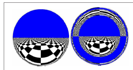
Figure 3: Alterations of Spacetime
