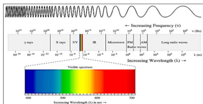
Figure 5: Electromagnetic Spectrum
