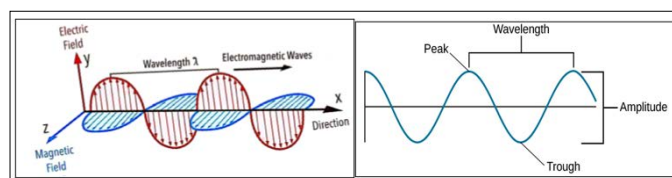
Figure 4: Electromagnetic Waves
