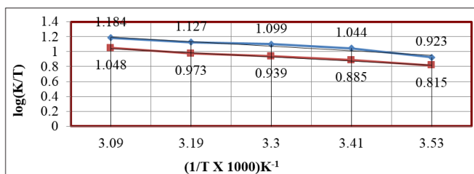
Figure 9: \log(K/T) Vs 1/T for copper with nanocoating of C(1) & SiC
