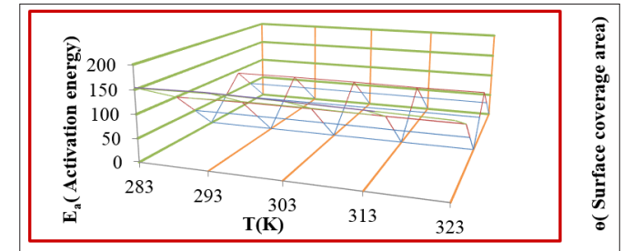
Figure 6: E_a Vs T, \theta for copper with nanocoating of C(1) & SiC
