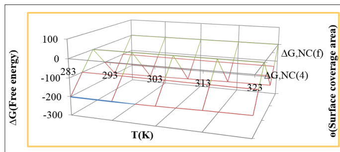
Figure 8: \Delta G Vs T, \theta for copper with nanocoating of C(1) & SiC
