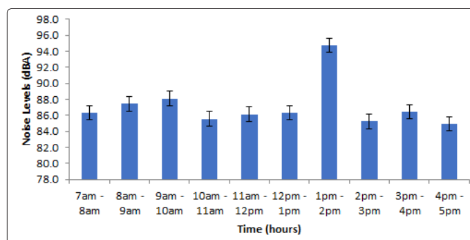
Figure 18: Hourly variation of Aircraft flyover noise (Location 3)
