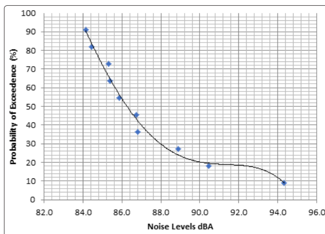
Figure 17: Probability of exceedance vs Noise levels (Location 2)
