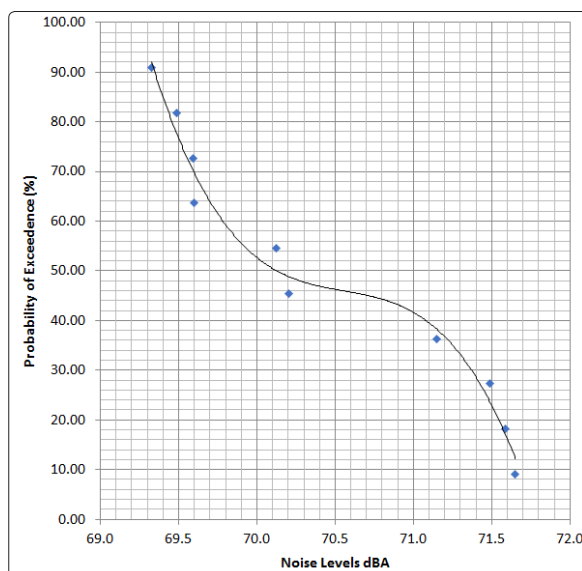
Figure 10: Probability of exceedance vs Noise levels (Location 3)
