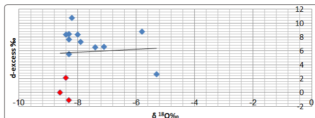
Figure 7: Relationship between \delta^{18}\text{O} and d-excess for Algerian C.I. with low d-excess values indicating the present-day recharge water (Filled Red squares). Originate from the present author
