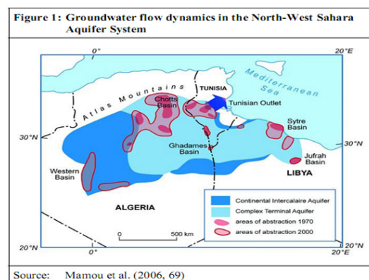
Figure 3: Location map and areal extent of North-Western Sahara Aquifer System (NWSAS)
