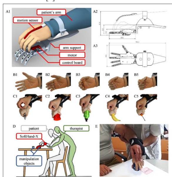
Figure 1: Robotic-Assisted Upper Limb Rehabilitation
