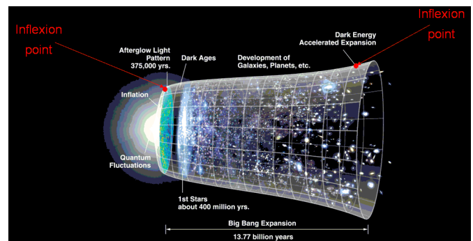
Figure 1: Expansion of Universe
