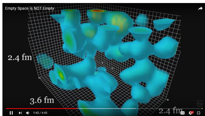
Figure 4: The Two Zones of the Universe
