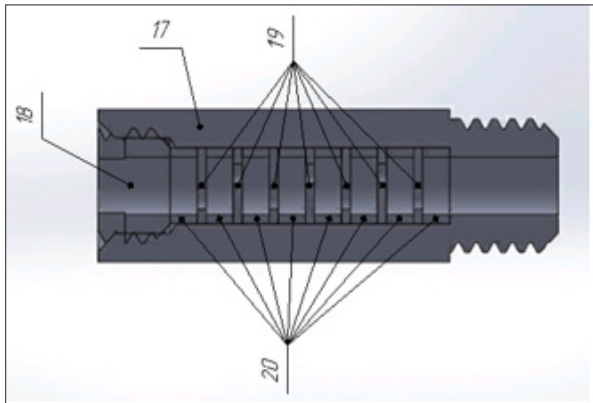
Figure 4: Throttle Package
