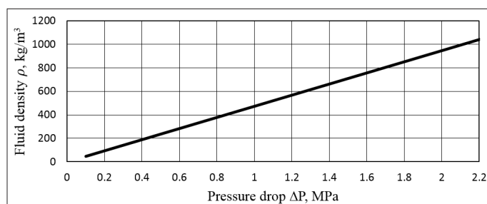
Figure 5: The Relationship Between the Pressure Drop and the Density of the Incoming Liquid
