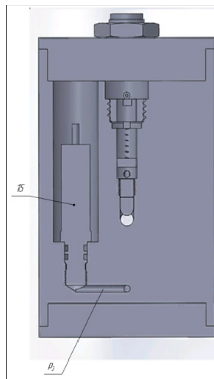
Figure 3: Cross-sectional View of the Pressure Sensor Setting
