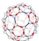
Alternating group A_5
