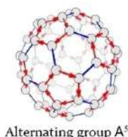
Alternating group A^5
