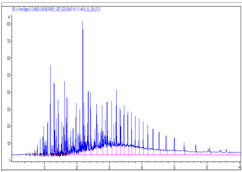
Figure 5: SBR Oil Sample HRGC FID Chromatogram
