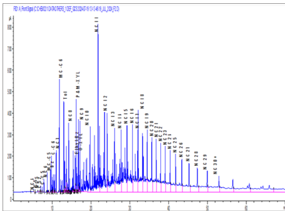
Figure 6: ORD Oil Sample HRGC FID Chromatogram
