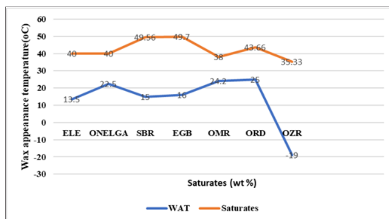
Figure 12: WAT and Saturates Profile for Waxy Crude Samples
