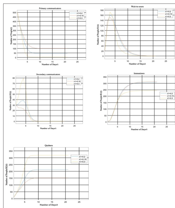
Figure 2.2: Impact of the transmission rate of primary communicators \lambda_1 on the five types of people
