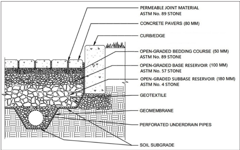
Figure 4: Typical Cross-Section of Structural Design of PICP [40]
