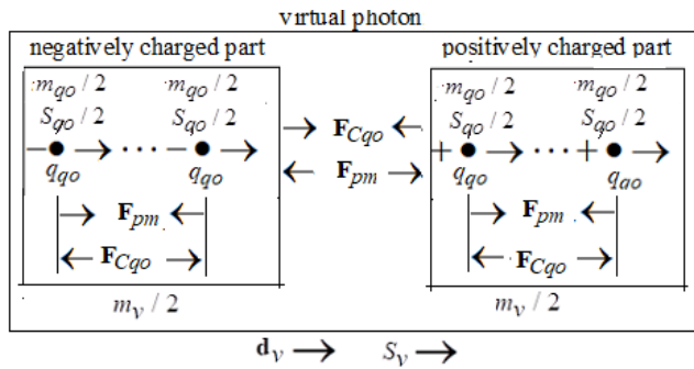
Figure 3: The structure of virtual photon: m_v , S_v and d_v are respectively mass, spin and electric dipole moment of virtual photon; m_{qo} , S_{qo} and q_{qo} are respectively mass, spin and charge determining the electric dipole moment of the quantum oscillators constituting the virtual photon; F_{Cqo} is a Coulomb force; F_{pm} is a pseudomagnetic force.
