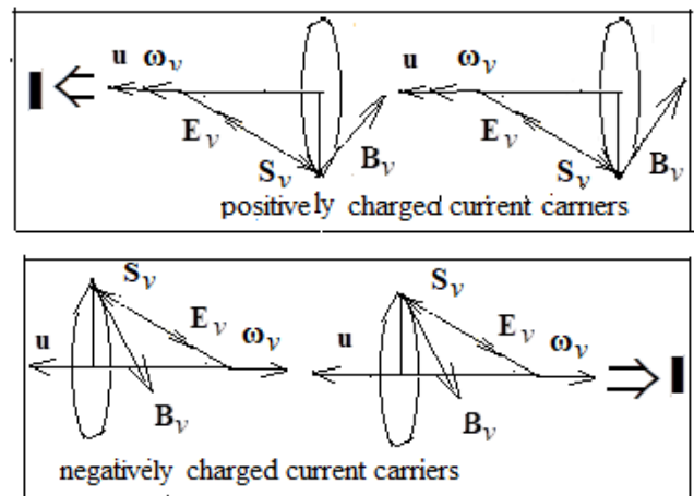
Figure 2: The characteristics of vortex lines consisting of virtual photons created by positively charged current-carriers (upper) and negatively charged current-carriers (below) forming current \mathbf{I} : velocities \mathbf{u} , spins \mathbf{S}_v , frequencies of precession \omega_v , electric components \mathbf{E}_v , magnetic components \mathbf{B}_v .
