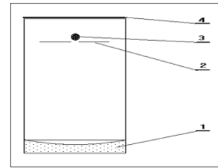
Figure 17: Schematic diagram of Kozyrev's telescope. 1 - focusing mirror, 2 - slit, 3 - detector, 4 - light-tight cover.
