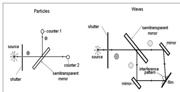
Figure 1: Experiments with Individual Photons on a Translucent Mirror
