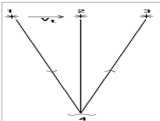
Figure 16: Past (1), present (2), and future (3) positions of an astronomical object. Photons of light emitted by an object at position (1) reach an observer (4) many years later. During this time, the object, moving perpendicular to the observer at velocity V_t , moves to position (2). If, at the moment of fixation, some of the light had been emitted for the observation point, it would have encountered the object at point (3).
