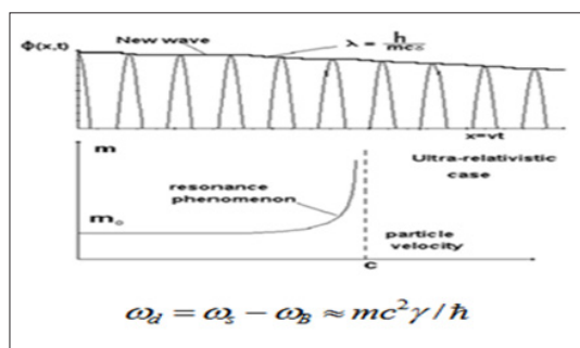
Figure 4: The emergence of a new low-frequency wave
