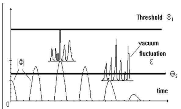
Figure 5: Quantum Measurements
