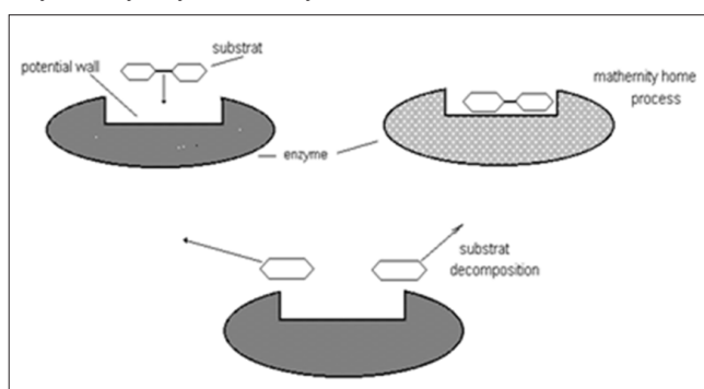
Figure 13: Polysaccharide splitting in the lysozyme molecule. Surprising results have been obtained for the catalytic decomposition
