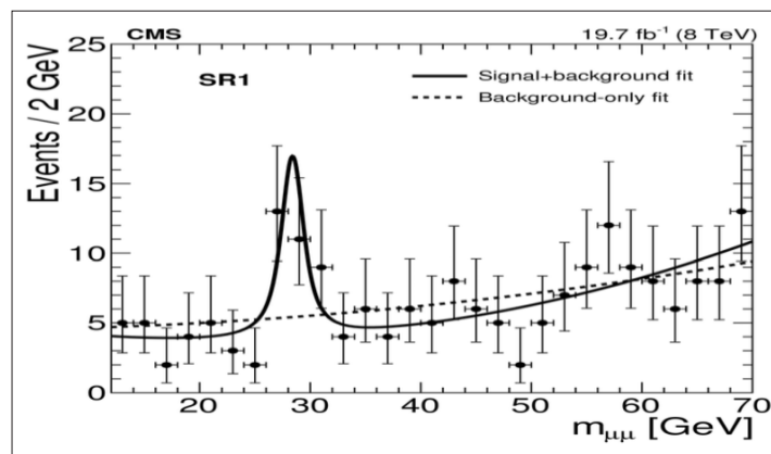
Figure 8: Energy peak at 28 GeV
