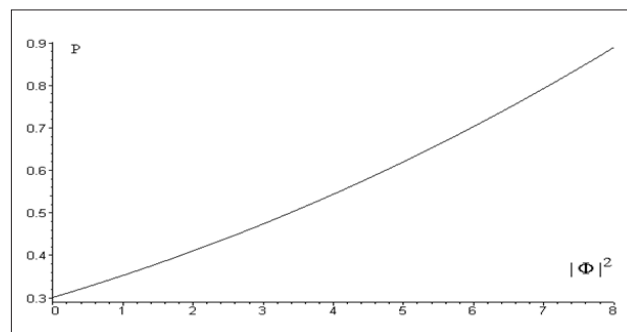
Figure 6: Probability of detecting a P particle in UQT
