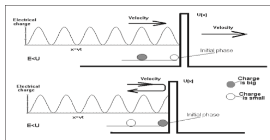
Figure 14: Illustration of the tunnel effect
