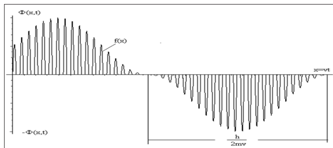
Figure 2: Wave packet behavior in a linearly dispersive medium (series of stroboscopic photographs).
