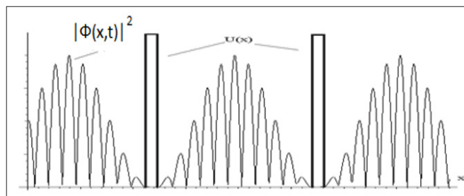
Figure 15: Visual representation of particles passing through two potentials barriers - a diagram of Maxwell's New Demon
