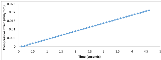
Figure 11: Compressive Strain versus Time for Al90Glass10 of 26.5 nm
