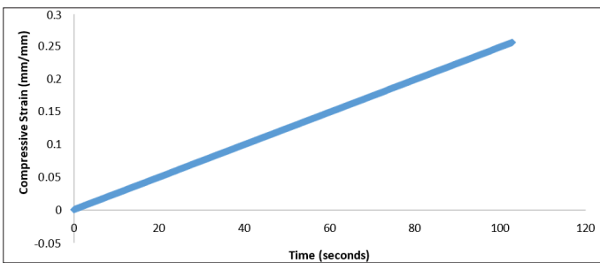
Figure 5: Compressive Strain with Time for Al30Glass70 of 26.5 nm
