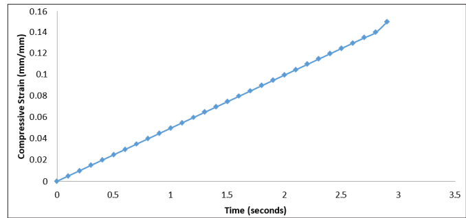
Figure 3: Compressive Strain with Time for Al10Glass90 of 26.5 nm
