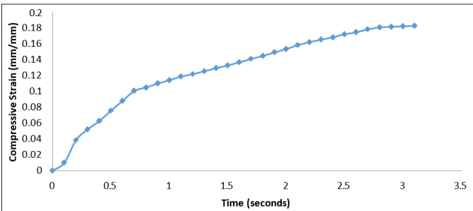
Figure 9: Compressive Strain with Time for Al70Glass30 of 26.5 nm
