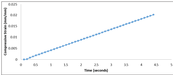
Figure 10: Compressive Strain versus Time for Al80Glass20 of 26.5 nm
