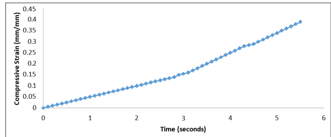
Figure 2: Compressive Strain with Time for Al0Glass100 of 26.5 nm
