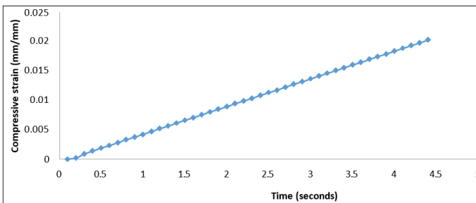
Figure 12: Compressive Strain versus Time for Al100Glass0 of 26.5 nm
