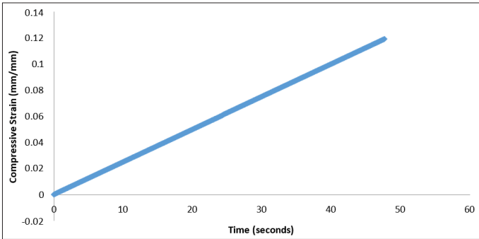
Figure 6: Compressive Strain with Time for Al40Glass60 of 26.5 nm
