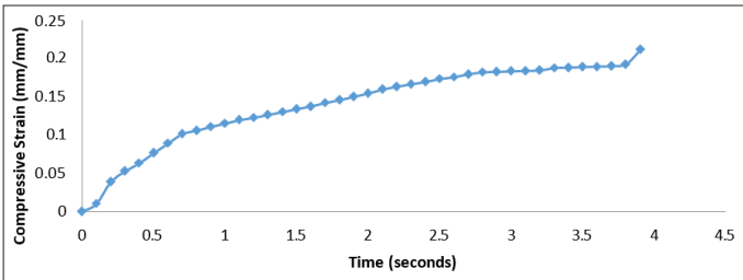
Figure 7: Compressive Strain with Time for Al50Glass50 of 26.5 nm
