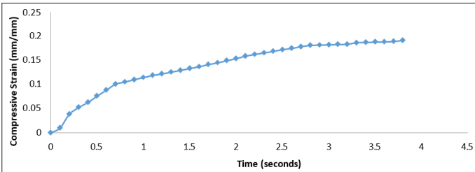
Figure 8: Compressive Strain with Time for Al60Glass40 of 26.5 nm
