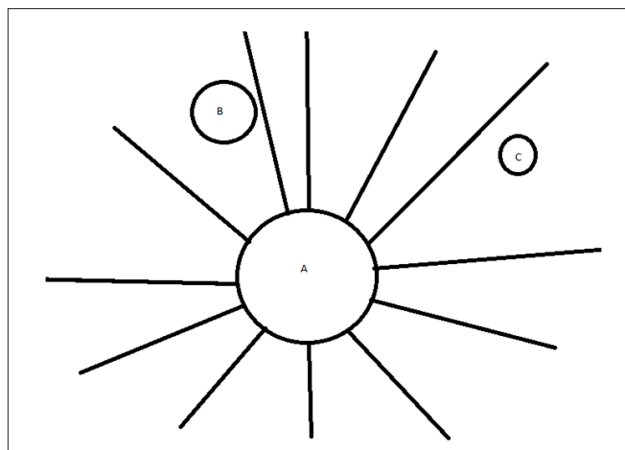
Figure 1: Radiation exiting the sun
