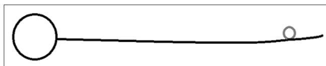
Figure 2: Bent Transmission Beams
