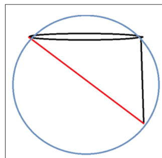
Figure 3: Gravity beam exiting at 45 degrees latitude. All such beams lead to a circle of exiting beam influence.
