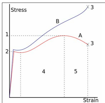
A stress-strain curve typical of structural steel.
