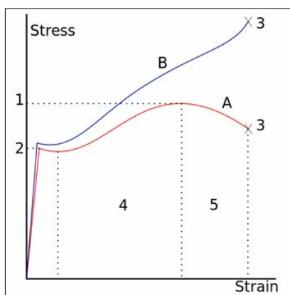
A Stress-Strain Curve Typical Of Structural Steel.
