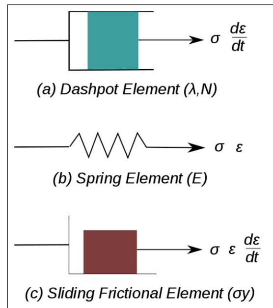
Figure 1: Elements used in one-dimensional models of viscoplastic materials
