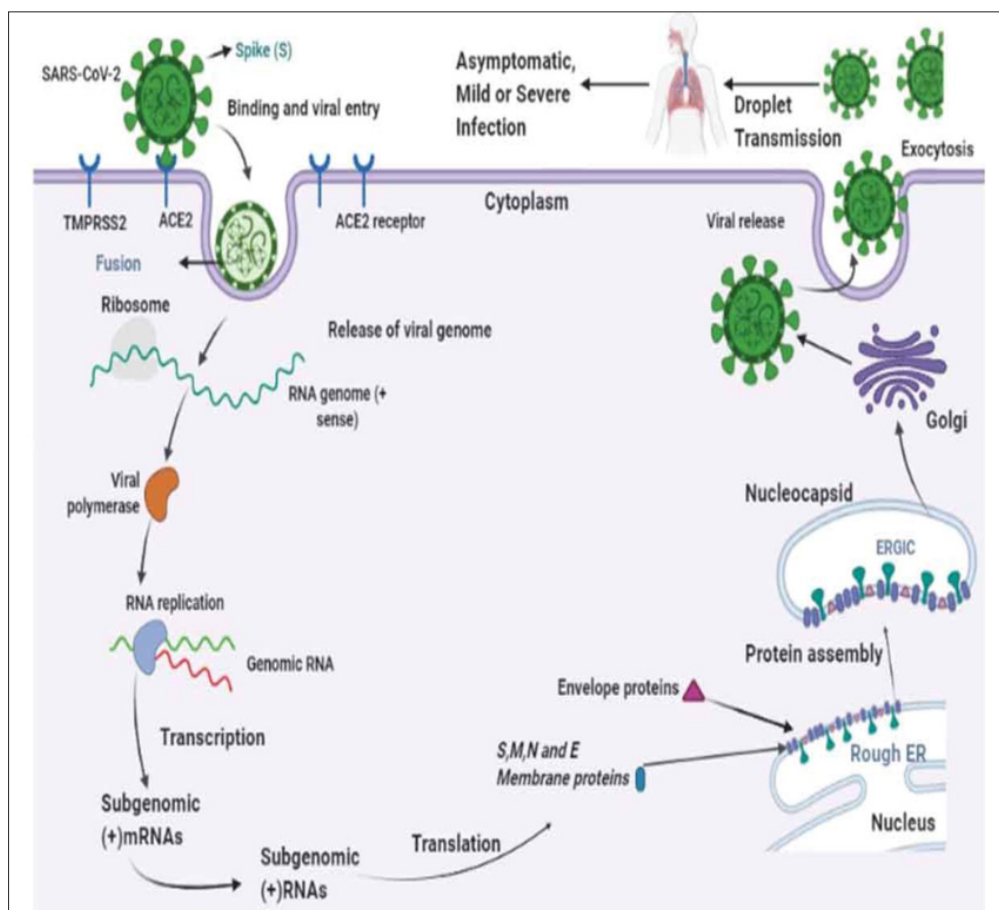
Figure 2: The transmission cycle of SARS-CoV-2 in the target cell. SARS-CoV-2 enters host cells by a membrane fusion or endosomal pathway. The S protein of SARS-CoV-2 is connected to the ACE2 receptor in the target cell and enters into the target cell by viral fusion. The SARS-CoV-2 virus produces its RNA polymerase that synthesizes virus RNAs, this virus RNA transcribes smaller subgenomic positive RNAs that are used to produce structural proteins. The proteins are completed in the membrane of the Endoplasmic Reticulum (ER) and are placed in a nucleocapsid, the progeny viruses are then released from the target cell through exocytosis by Golgi vesicles and are transferred by droplets causing infections.
