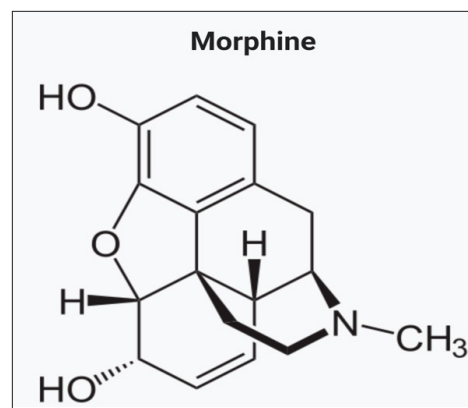
Figure 3: Chemical structure of morphine
