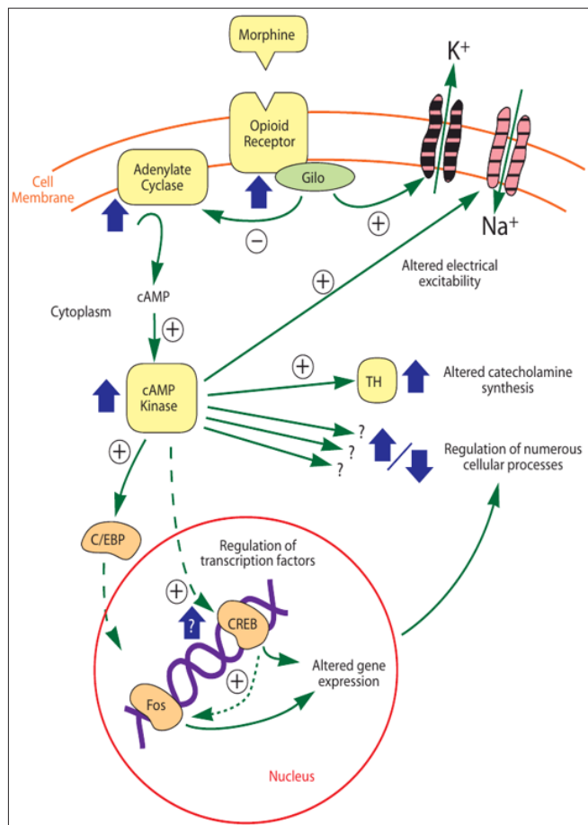
Figure 4: Intracellular morphine activation
