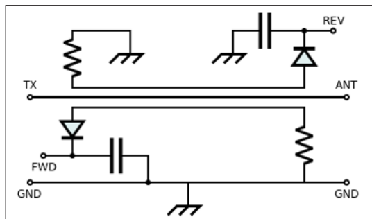
Figure 2: A Simple Directional SWR Meter
