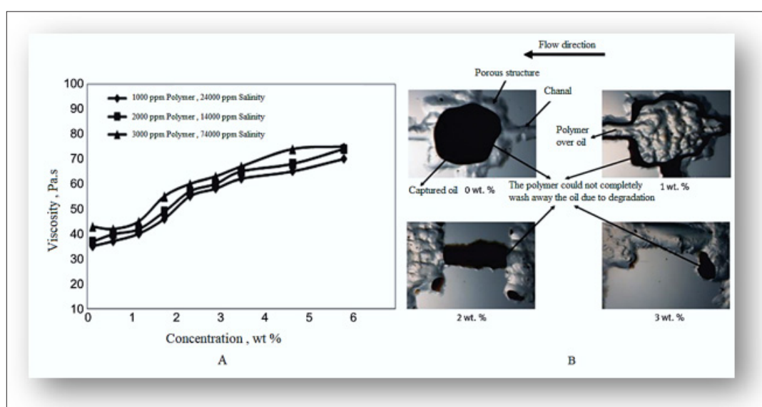
Figure 4: An analysis of the impact of nanoparticles on polymer flooding: A - Silica nanoparticle concentration influences the viscosity of polymer solutions at different salinities and polymer concentrations, B - Residual oil and polymer solution distribution at the pore scale during polymer flooding with a 1,000 ppm polymer solution (24,000 ppm salinity) and varying silica nanoparticle concentrations.
