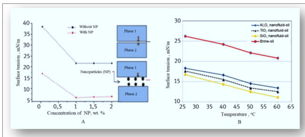
Figure 2: Formation Interfacial Tension . A - Interfacial Tension between two Liquid Phases, With and without the Presence of Nanoparticles. B- At the Oil-Water Interface, Observed at Various Temperatures and at Atmospheric Pressure.
