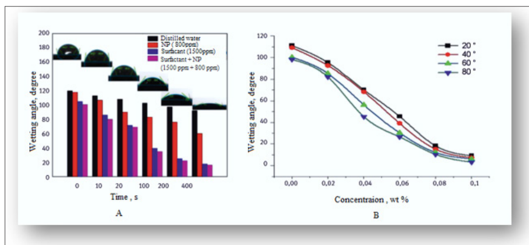
Figure 3: Wettability graphs: A) Wetting angles of various samples, including distilled water, nanoparticles (800 ppm), surfactants (1,500 ppm), and a combination of surfactants and nanoparticles (1,500 ppm + 800 ppm); B) The influence of silicon dioxide nanoparticle concentration on the wetting angle. Distilled water reduced the contact angle from 120° to 92°, indicating that the rock surface is moderately wettable. The SiO 2 nanofluid reduced the contact angle to 60 ° from 118°, indicating that the rock surface is preferentially wetted by water. The surfactant solution changed the contact angle from 105 to 17°, indicating that the rock surface is predominantly water-wet. The contact angle value decreased from 100.2 to 16.2° for the surfactant-SiO 2 nanofluid (1,500 ppm + 800 ppm) suspension. The results indicate that the presence of SiO 2 nanoparticles in the surfactant solution provides better overall wettability properties. The presence of SiO 2 nanoparticles can influence the strong physicochemical interactions that occur at the liquid-solid interfaces, resulting in a favourable change in wettability for oil recovery. Many studies have focused on identifying the concentration ranges of nanoparticles and their effects on wettability modification [33-36]. Most studies have shown that with increasing nanoparticle concentration, rock wettability improves due to repulsive forces. Other studies, on the contrary, indicate that excessive concentrations can lead to pore blockage and increased operating costs [37-40]. Therefore, an ideal concentration is preferable to control wettability. The results indicate that increasing the concentration of nanoparticles results in a consistent decrease in the contact angle at all temperatures. The ideal concentration is 0.1 wt%, as shown in Figure 3b. Most of the measured contact angle values fall below 70°, which provides strong evidence that nanoparticles can effectively alter the wettability from hydrophobic to hydrophilic [41-44]. Polymers have been successfully used as viscosity-controlling agents to improve recovery efficiency [45-48]. In formations with high temperatures, pressures, and salinity, polymer fluids can decompose, which reduces their viscosity and displacement efficiency. The use of nanoparticles can increase the viscosity of the displacing fluid without reducing stability. The effect of silica nanoparticle dispersions on oil displacement by polymers with different fluid mineralisation is studied. Adding silica nanoparticles to the solution increased stability and showed greater efficiency compared to water and polymer (without nanoparticles) displacement. The study was conducted to investigate the dependence of the viscosity of the injected solutions on the concentration of nanoparticles (Figure. 4A).
