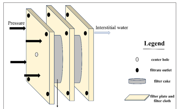
Figure 3: Principle of Plate and Frame Filter Press
