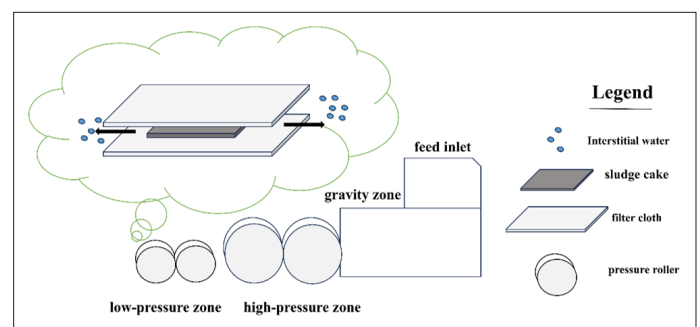
Figure 4: Schematic Diagram of Belt Filter Press
