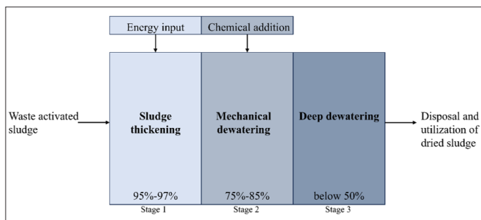
Figure 2: Flow Chart of Sludge Dewatering
